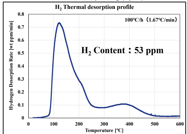
Electro Ni plating (5 \mu m)
